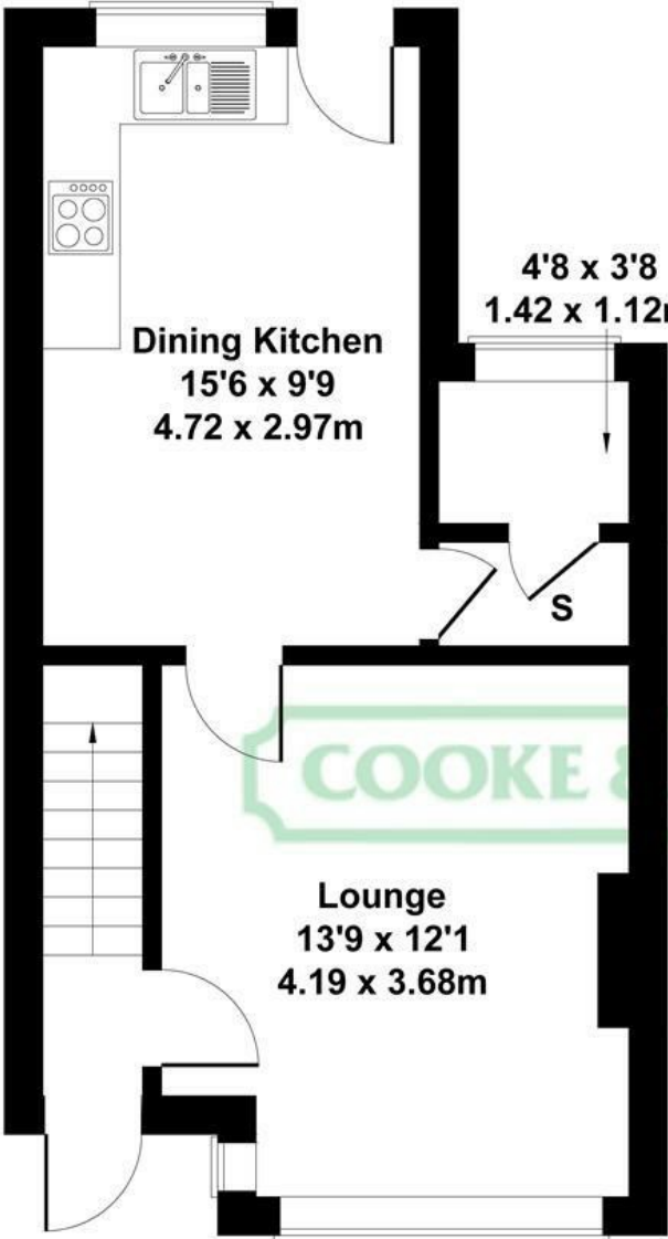
GROUND FLOOR
